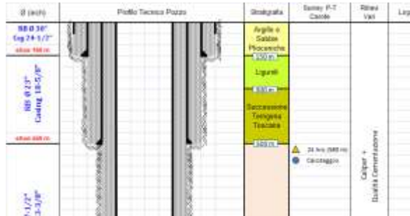
ITALY – ZERO-EMISSION PLANTS DRILLING PROGRAM
